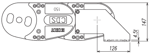
[ Fixed Bracket (F/EB) ]
