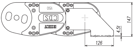
[ Moving Bracket (M/EB) ]
