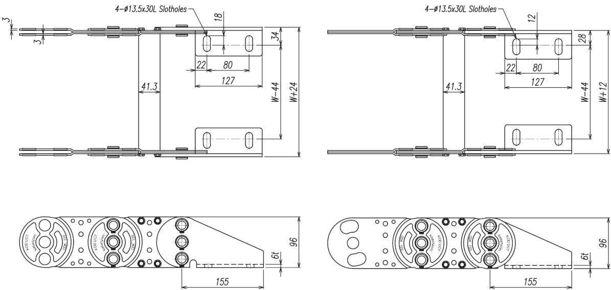
[ Fixed Bracket (F/EB) ]
