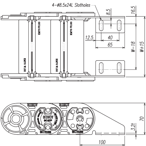
[ Moving Bracket (M/EB) ]
